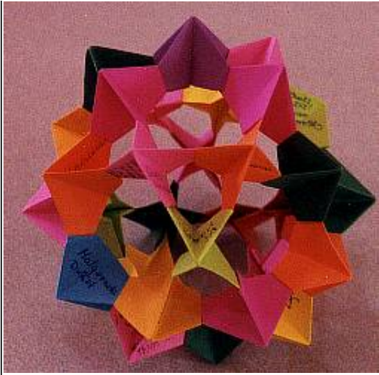
The icododecaheron, triangular face.
