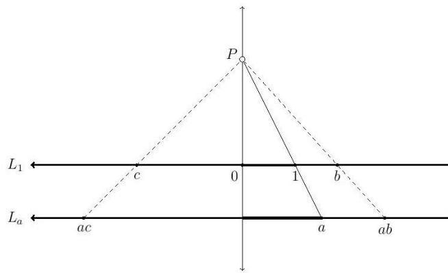
Figure 1. Multiplication by a with a > 1 .
